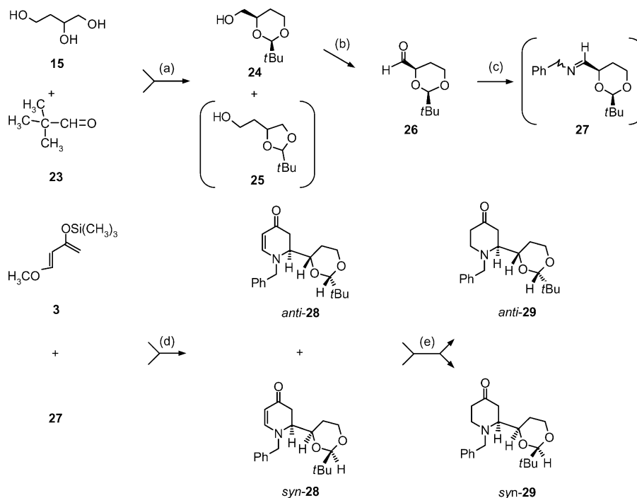
Scheme 3. (a) THF, TosOH, reflux, 23 h, 24 : 41%; 25 : 38%; (b) \text{CH}_2\text{Cl}_2 , (\text{COCl})_2 , DMSO, \text{NEt}_3 , -78^\circ\text{C} , 84%; (c) \text{HC}(\text{OCH}_3)_3 , \text{BnNH}_2 , room temp., 16 h; (d) THF, \text{Yb}(\text{OTf})_3 , 0^\circ\text{C} , 4 h, then room temp., 16 h, 90%; (e) THF, \text{LiBHET}_3 , \text{BF}_3\cdot\text{OEt}_2 , -78^\circ\text{C} , 60 min, 72%. All compounds are racemic, only one enantiomer is shown.
