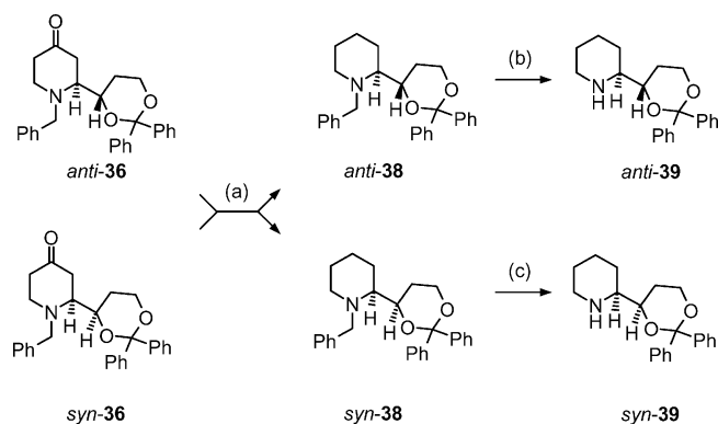
Scheme 6. (a) MeOH, p -toluenesulfonylhydrazide, reflux, 2 h, then \text{NaBH}_4 , reflux, 6 h, anti -38: 13%; syn -38: 12%; (b) MeOH, Pd/C, \text{H}_2 (balloon), room temp., 1 h, 97%; (c) MeOH, THF, Pd/C, \text{H}_2 (balloon), room temp., 1.5 h, 95%. All compounds are racemic, only one enantiomer is shown.
