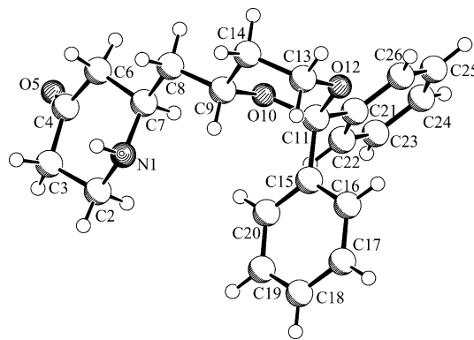
Figure 4. X-ray crystal structure analysis of anti -14.
