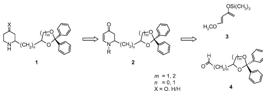
Figure 2. Strategy for the synthesis of novel ring and side chain homologues of dexoxadrol.
