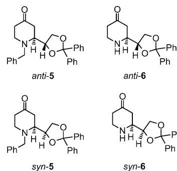
Figure 3. Dexoxadrol derivatives with an additional oxo group in the 4-position of the piperidine moiety (oxodexoxadrol; compounds are racemic, only one enantiomer is shown).
