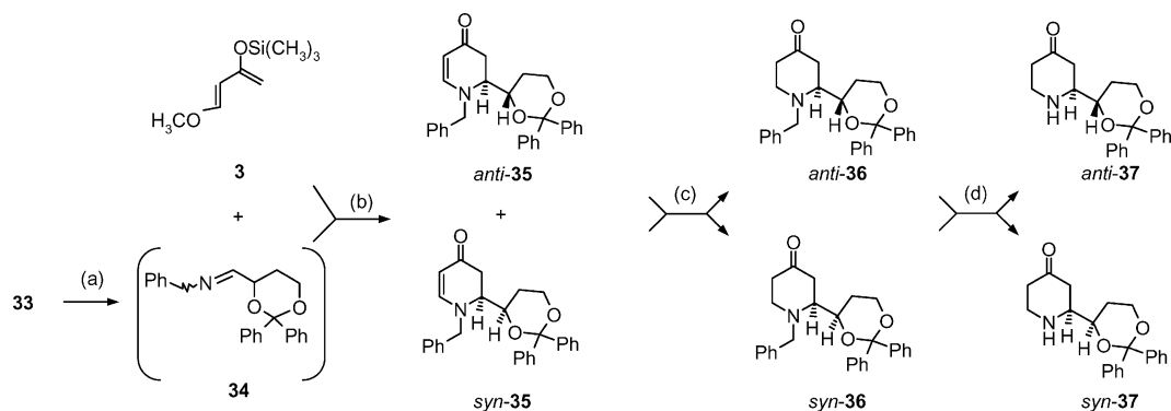
Scheme 5. (a) \text{HC}(\text{OCH}_3)_3 , \text{BnNH}_2 , room temp., 3 h; (b) THF, \text{Yb}(\text{OTf})_3 , -15^\circ\text{C} , 1 h, then room temp., 16 h, 92%; (c) THF, \text{LiEt}_3\text{H} , \text{BF}_3\cdot\text{OEt}_2 , -78^\circ\text{C} , 60 min, 82%; the diastereomers anti -36 and syn -36 were separated by preparative HPLC; (d) MeOH, Pd/C, \text{H}_2 (balloon), room temp., 4.25 h, anti -37: 55%; syn -37: 34%. All compounds are racemic, only one enantiomer is shown.
