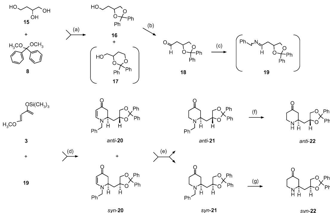
Scheme 2. (a) THF, TosOH, reflux, 4 h, 64%; (b) CH 2 Cl 2 , (COCl) 2 , DMSO, NEt 3 , -78 °C, 37%; (c) HC(OCH 3 ) 3 , BnNH 2 , room temp., 2.5 h; (d) THF, Yb(OTf) 3 , -10 °C - 0 °C, 4 h, then room temp. 16 h, 41%; (e) THF, LiBHET 3 , BF 3 ·OEt 2 , -78 °C, 90 min, anti - 21 : 49%; syn - 21 : 16%; (f) MeOH, Pd/C, H 2 (balloon), room temp., 3 h, 97%; (g) MeOH, Pd/C, H 2 (balloon), room temp., 3.5 h, 89%. All compounds are racemic, only one enantiomer is shown.
