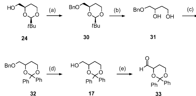
Scheme 4. (a) THF, \text{BnBr} , \text{Bu}_4\text{N}^+\text{I}^- , NaH, room temp., 16 h, 86%; (b) MeOH, Amberlyst® 15, reflux, 2 h (3x), 93%; (c) THF, 8 , TosOH, reflux, 19 h, 89%; (d) EtOAc, Pd/C, \text{H}_2 (balloon), room temp., 1.75 h, 88%; (e) \text{CH}_2\text{Cl}_2 , (\text{COCl})_2 , DMSO, \text{NEt}_3 , -78^\circ\text{C} , 76%. All compounds are racemic, only one enantiomer is shown.
