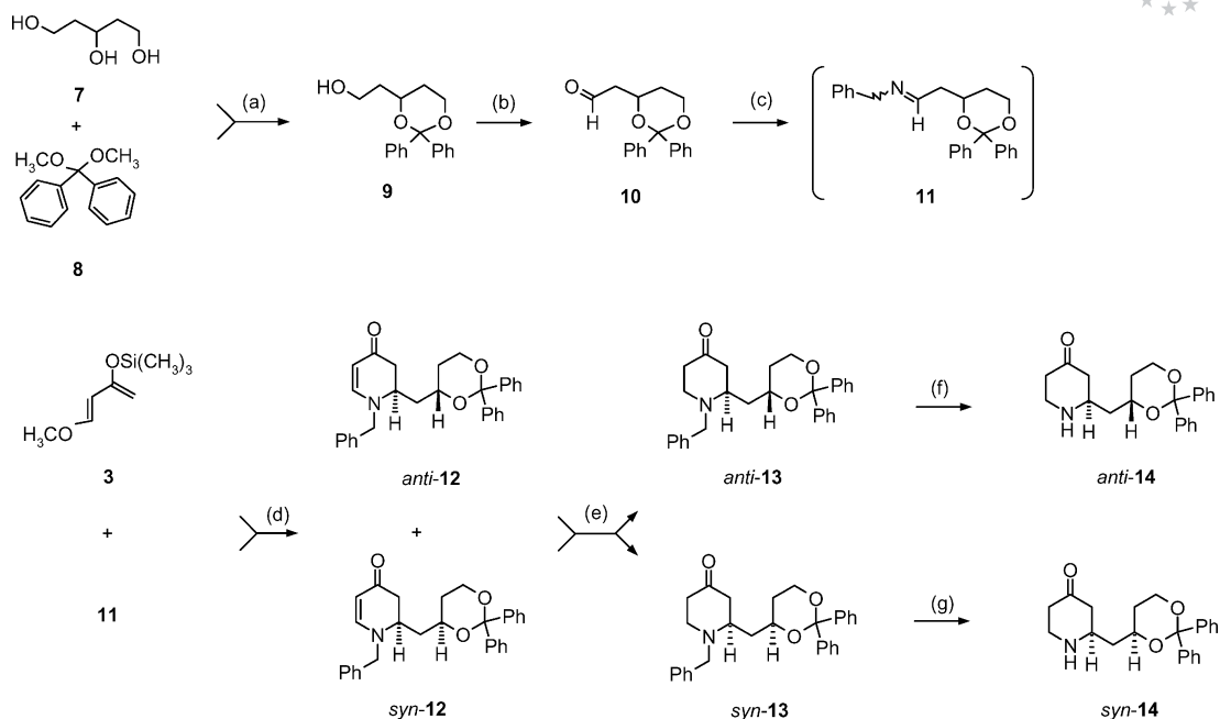
Scheme 1. (a) THF, TosOH, reflux, 7 h, 91%; (b) \text{CH}_2\text{Cl}_2 , (\text{COCl})_2 , DMSO, \text{NEt}_3 , -78^\circ\text{C} , 87%; (c) \text{HC}(\text{OCH}_3)_3 , \text{BnNH}_2 , room temp., 5 h; (d) THF, \text{Yb}(\text{OTf})_3 , 0^\circ\text{C} , 4 h, then room temp., 16 h, 74%; (e) THF, \text{LiBHET}_3 , \text{BF}_3\cdot\text{OEt}_2 , -78^\circ\text{C} , 60 min, anti - 13 : 60%; syn - 13 : 23%; (f) MeOH, THF, Pd/C, \text{H}_2 (balloon), room temp., 3.5 h, 89%; (g) MeOH, Pd/C, \text{H}_2 (balloon), room temp., 5 h, 88%. All compounds are racemic, only one enantiomer is shown.
